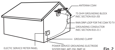
Example of Antenna Grounding as per NEC - National Electrical Code
